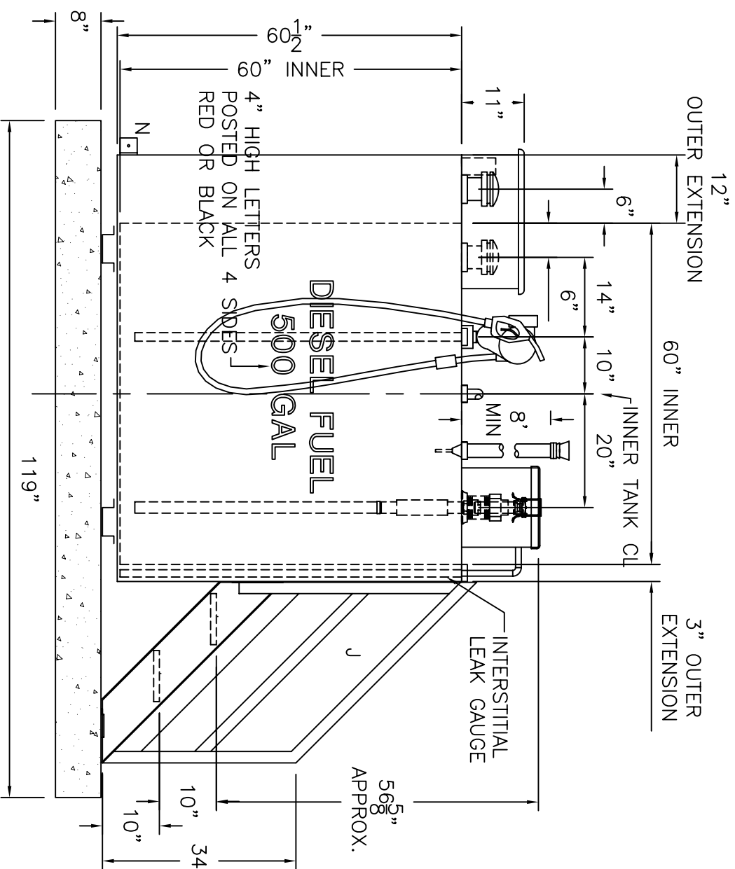
ELEVATION "A"
